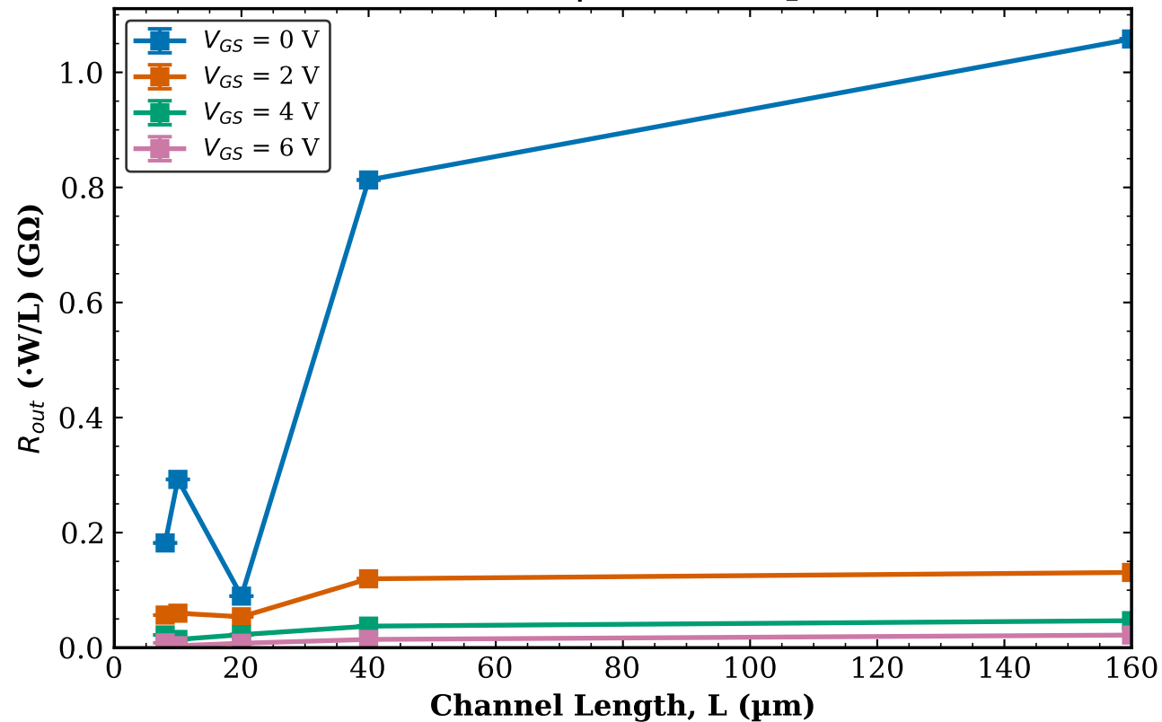
TFT1 Transistor 1 R_{out} vs L | W = 100\text{ }\mu\text{m}
